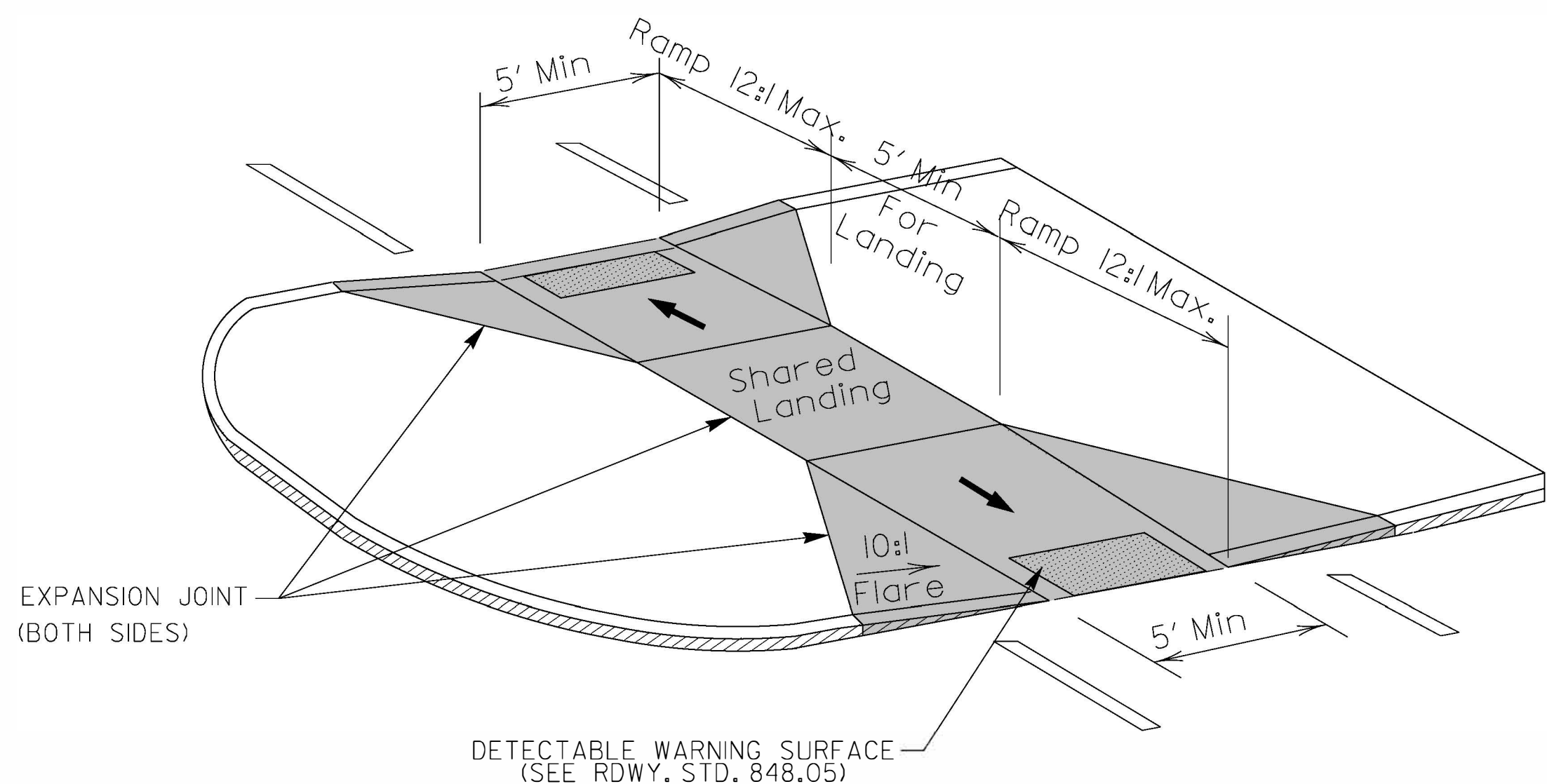
MEDIAN ISLAND TYPE 8 CURB RAMPS
